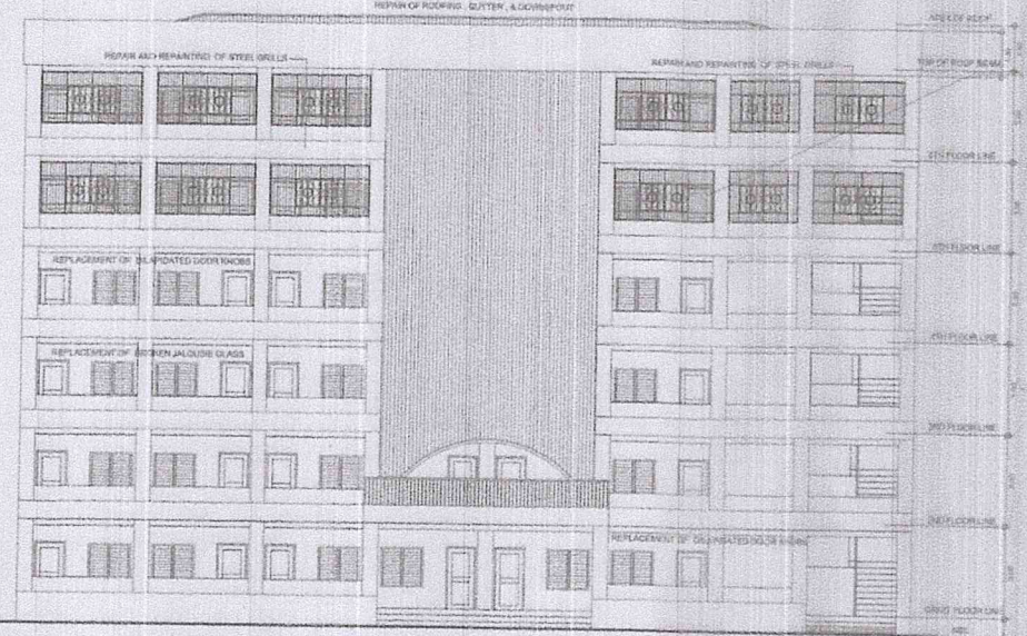
6-STOREY BUILDING FRONT ELEVATION SCALE: 1:100
