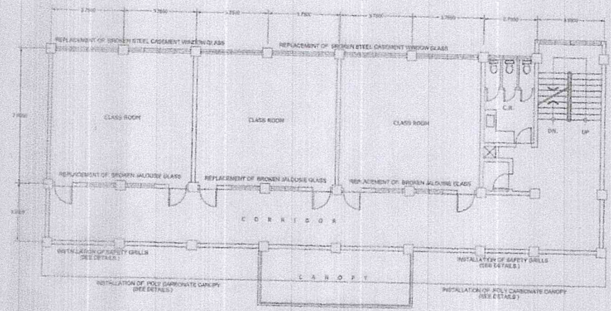
TYP. FLOOR PLAN SCALE: 1:1000
